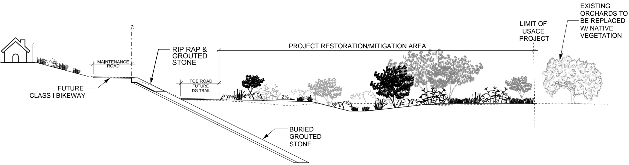
TYPICAL SECTION USACE REACH 9 BANK PROTECTION IMPROVEMENTS SCALE: N.T.S.
